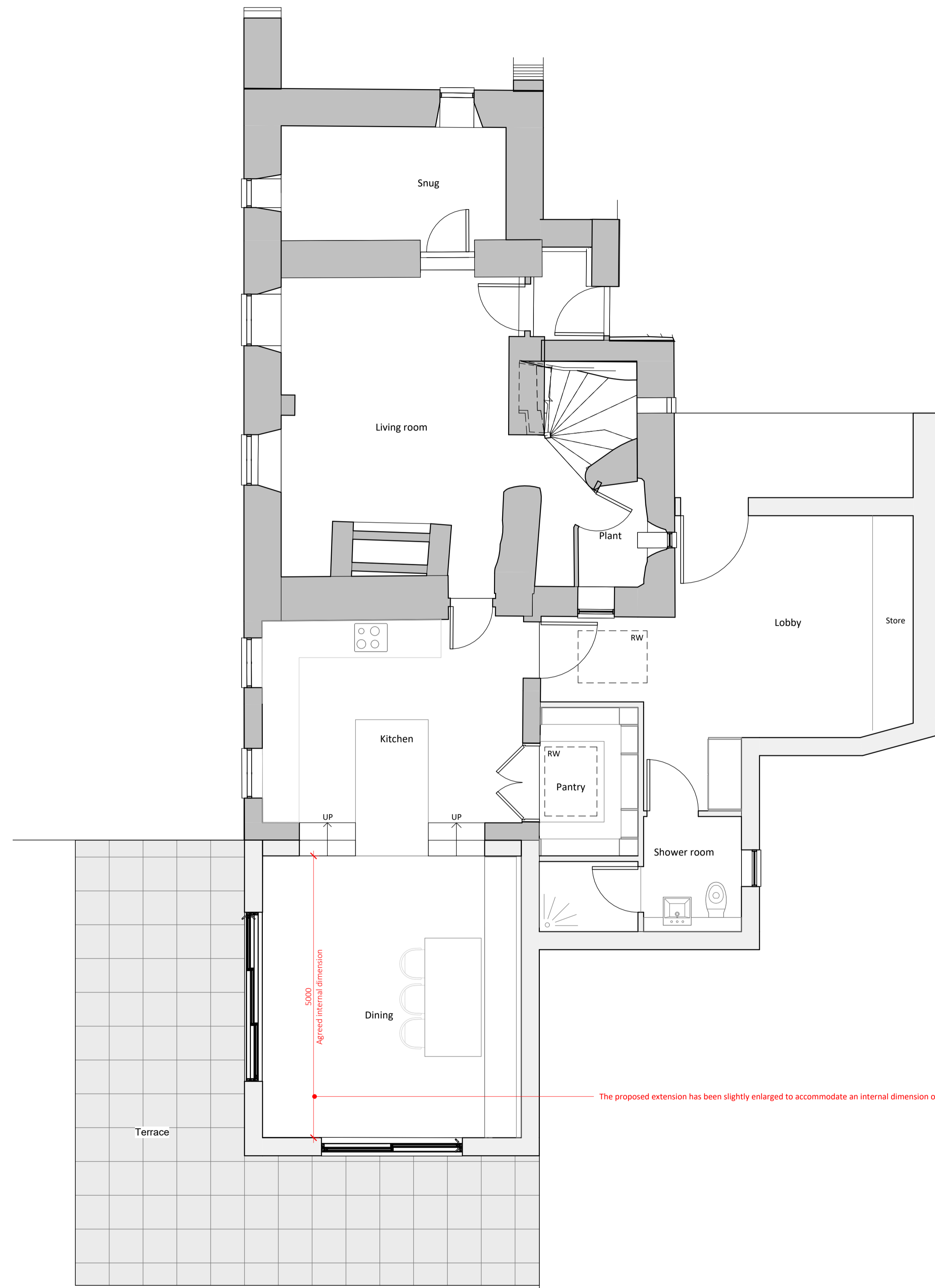
Proposed Level 00 1 : 50
